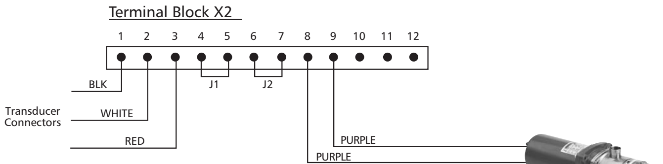
Motor Thermistor Connection
