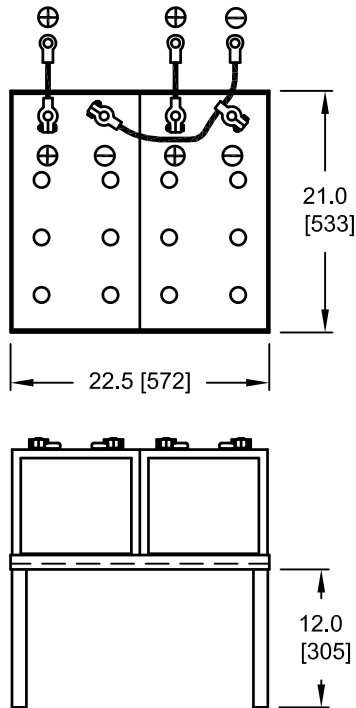
FIG. 1 12V NEG. GROUND (2 BATTERIES)
