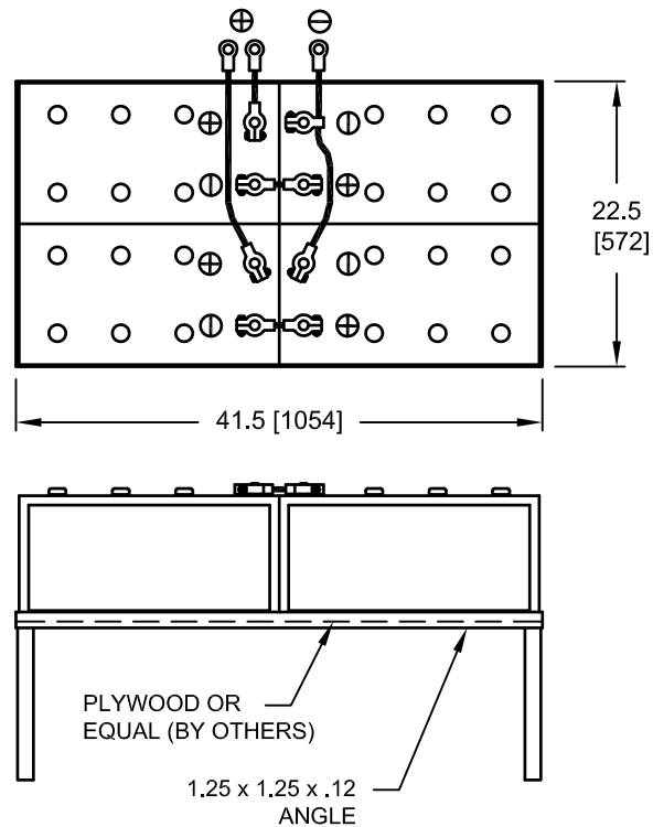
FIG. 2 24V NEG. GROUND (4 BATTERIES)
