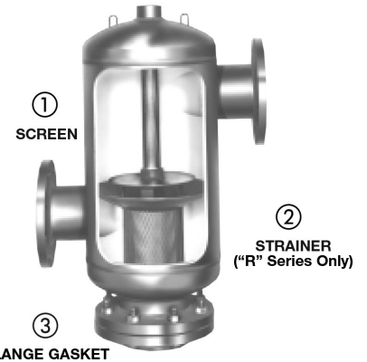
"R" Series with strainer manufactured before March 2010 for 2" and 2 1/2" and before June 2007 for 3"-12"
